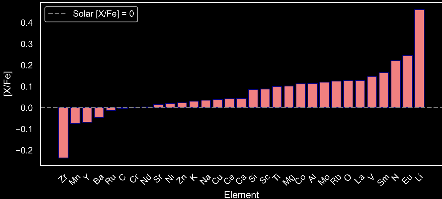
Abundance Pattern for GALAH Star Field [5] (N=177)
