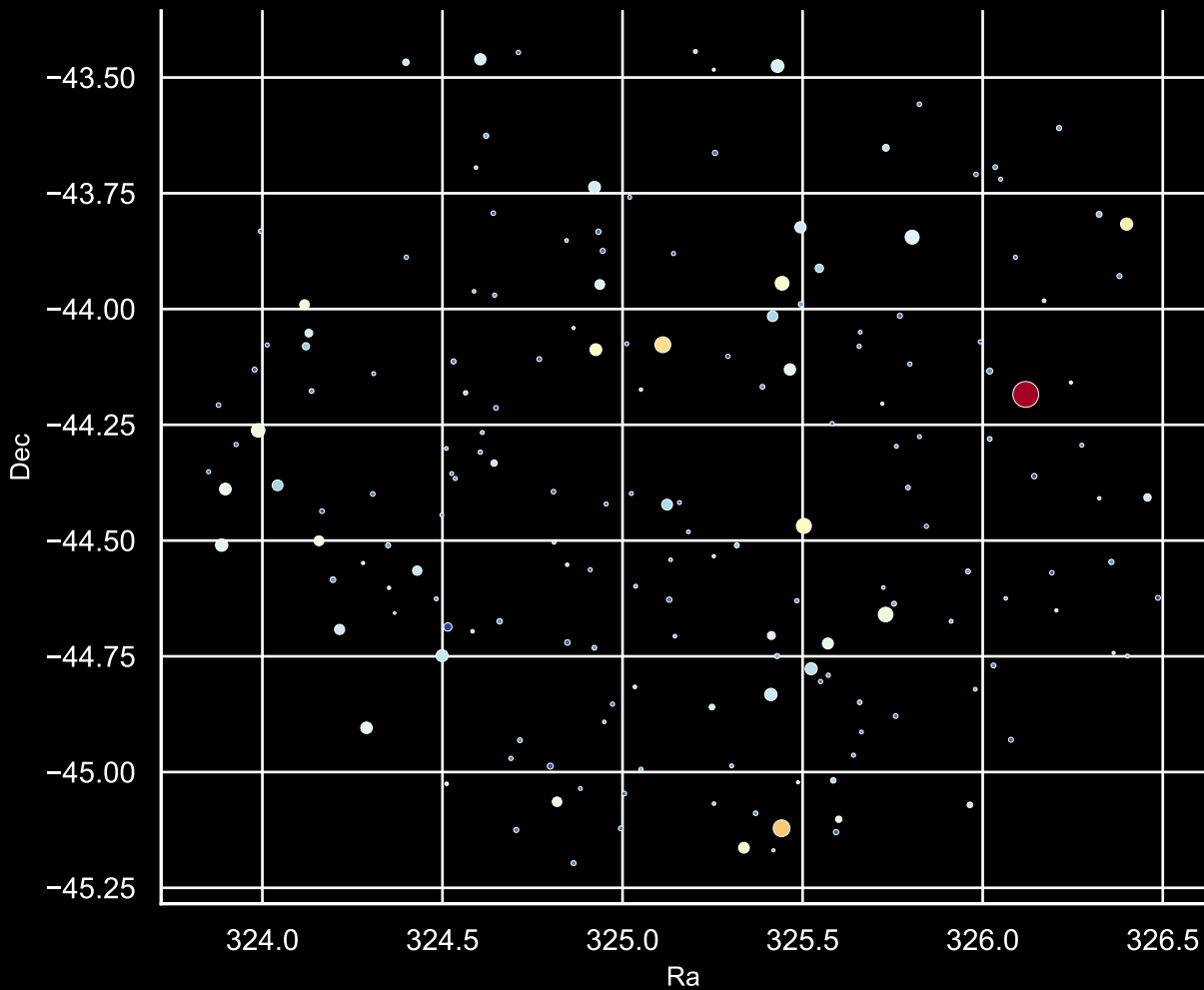
Field [5] Ra [325.17] Dec [-44.39] Stars: 177
