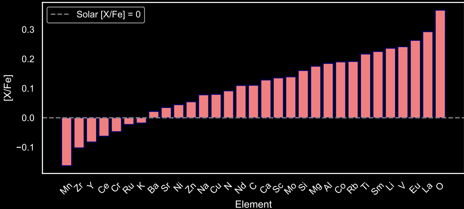
Abundance Pattern for GALAH Red Giants: Star Field [5] (N=42)
