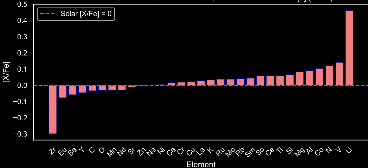
Abundance Pattern for GALAH Main Sequence Stars: Star Field [5] (N=82)
