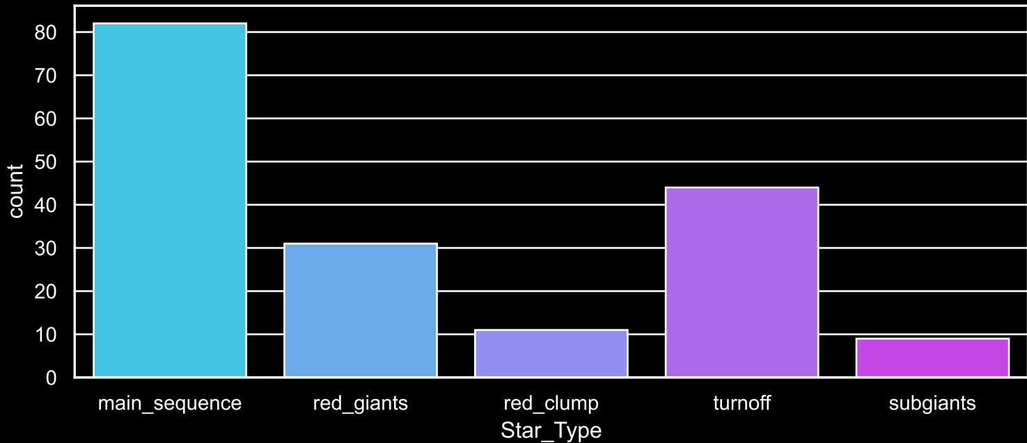
Field [5] Count plot of Star Type
