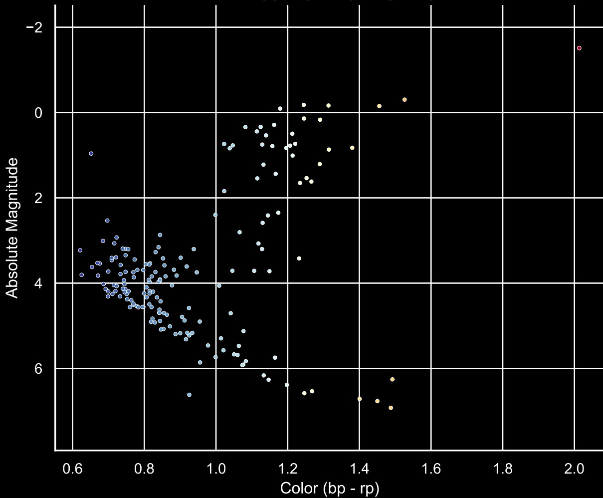
GALAH Hertzprung-Russel Diagram Field [5] Ra [325.17] Dec [-44.39]
